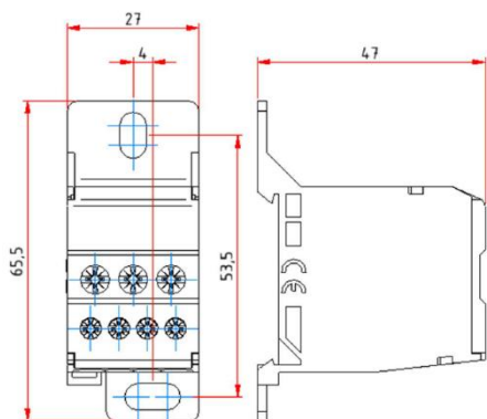
Assembly Details | Montage
